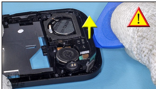
16. Use the SRT-6 to remove carefully the MONO ANTENNA ASSY. Avoid damaging the gaskets.
