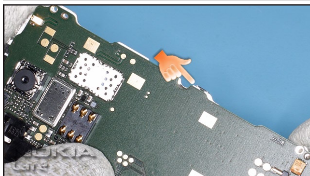
12. Unlock the PWB and carefully open the parts.
