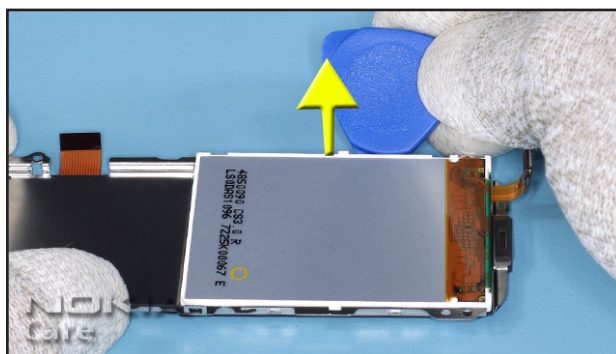
14. Remove the LCD from the C-COVER.
