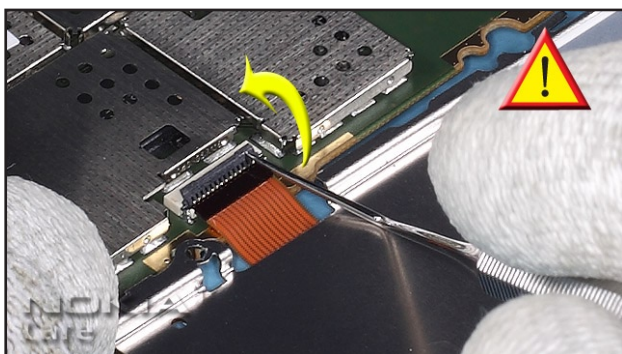
13. Take special care to the flex connector. Gently unlock the flex and take it out.
