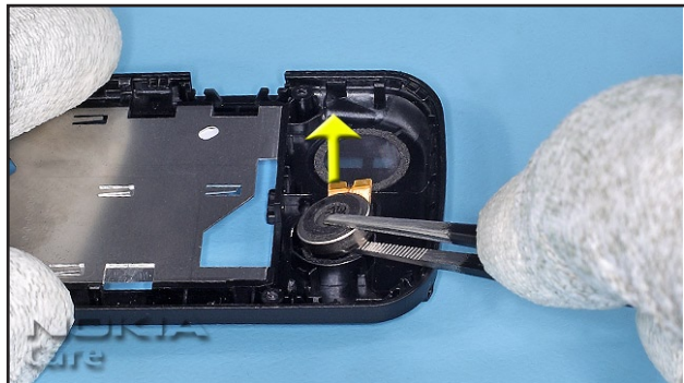
18. Carefully remove the VIBRA MOTOR. Avoid damaging the gasket.
