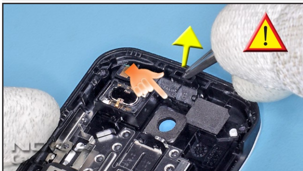
15. Unlock the IHF ANTENNA MODULE and remove it from the D-COVER.
