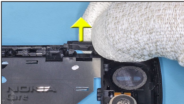
17. Remove the CAMERA KEY.
