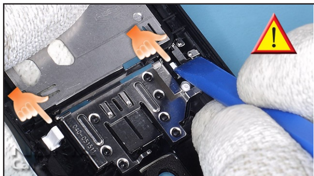
20. The B-DECO COVER is glued onto the D-COVER. Carefully unlock the clips from the B-DECO COVER.
