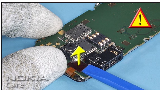
11. Carefully open the LCD connector.
