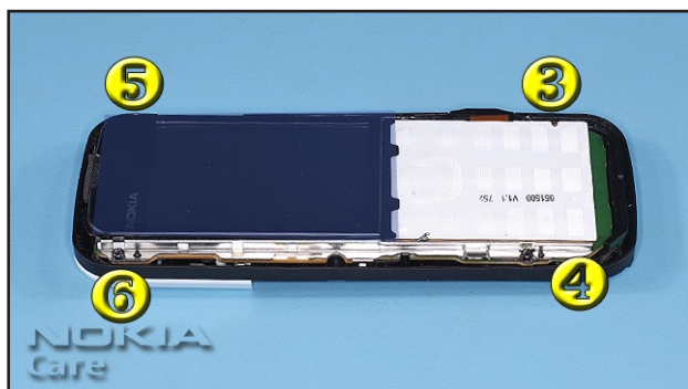
9. Undo the Torx PLUS size 4 SCREWS in the order shown.
