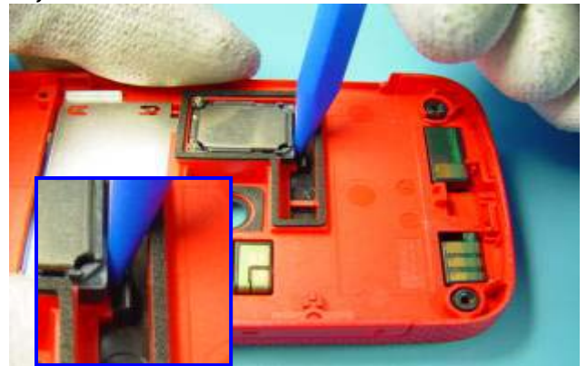
28) Ease out and remove the IHF SPEAKER.
