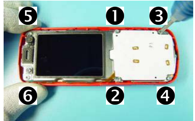
14) Unscrew the Torx Plus size 6 screws in the order shown.
