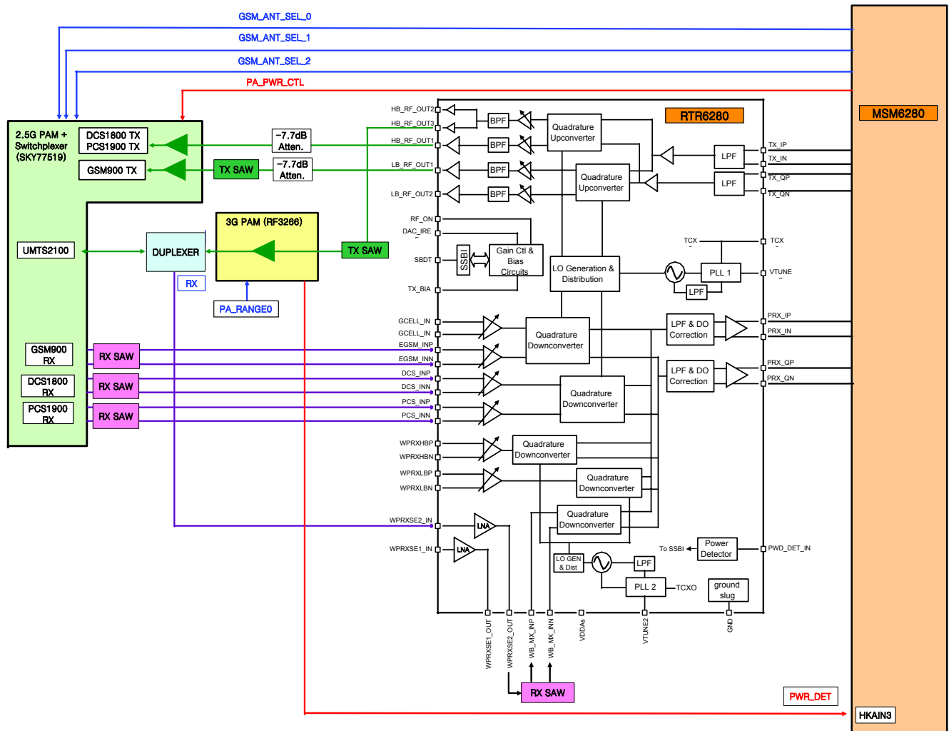
SGH-U900 RF Block Diagram
