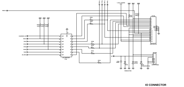
IO CONNECTOR
