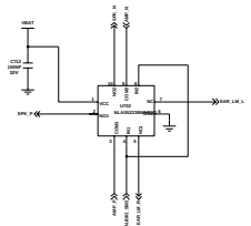
EARPHONE SWITCH
