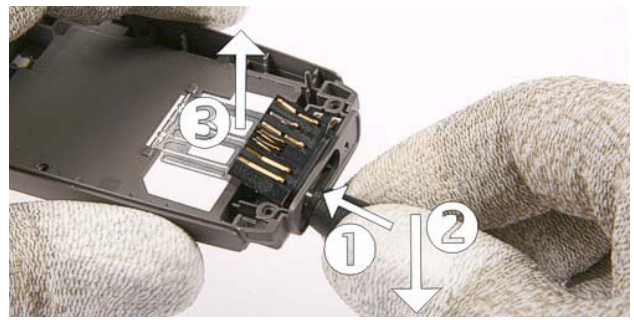
20.) Press out the Easy Flash Connector by using the DC-plug.
