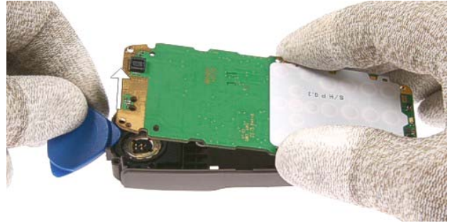
18.) Lift the Engine Module a bit with the SRT-6 and remove it from the D-Cover Assy.
