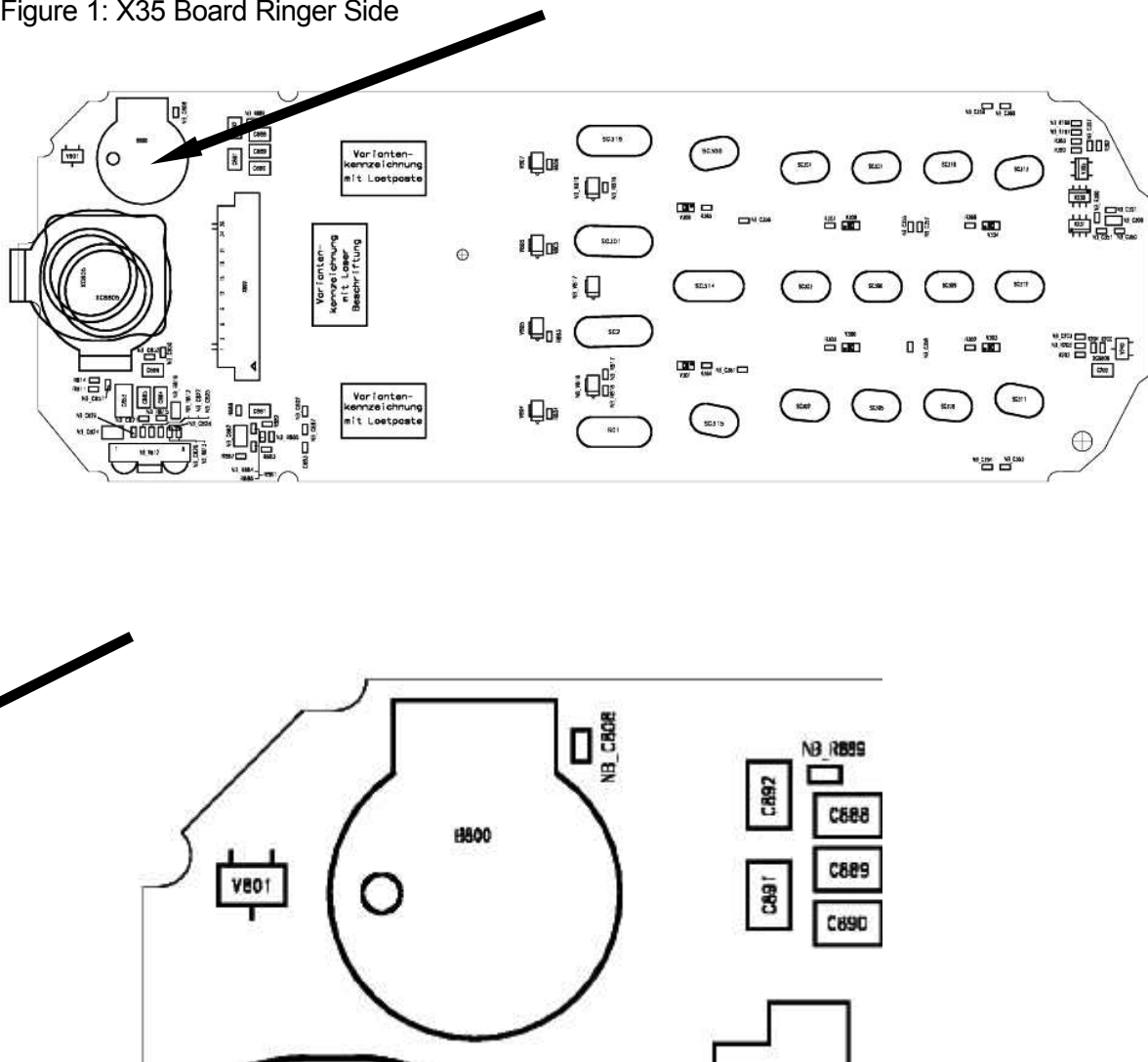
Figure 1: X35 Board Ringer Side
