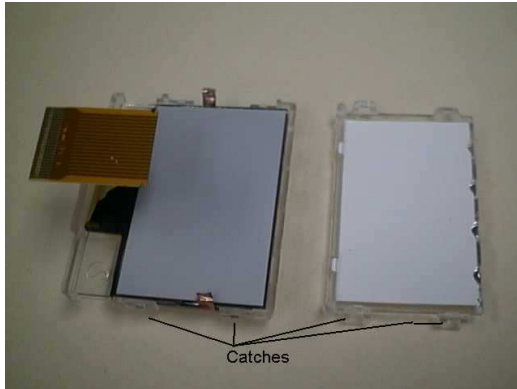
PHOTO 2.19 Disassembly Display Module – STEP
