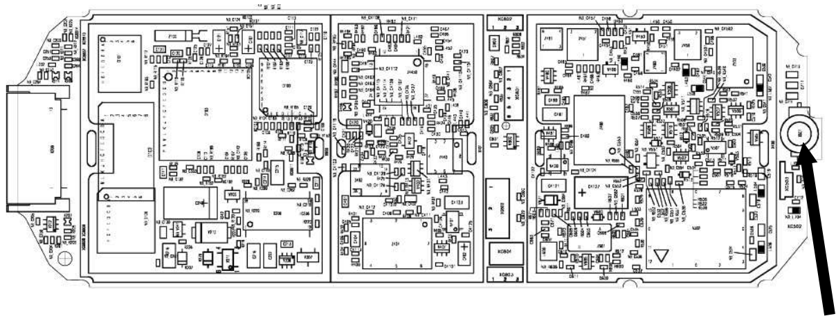
Figure 1: X35 Board Antenna Connector Side (Top View)
