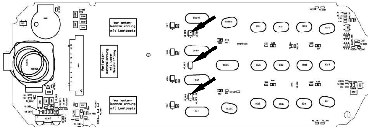
Figure 4: S35 board display LED placement and polarity
