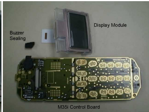
PHOTO 2.15 Disassemble Control Board Assy – STEP 2 PHOTO 2.16 Disassemble Control Board Assy – STEP 3
