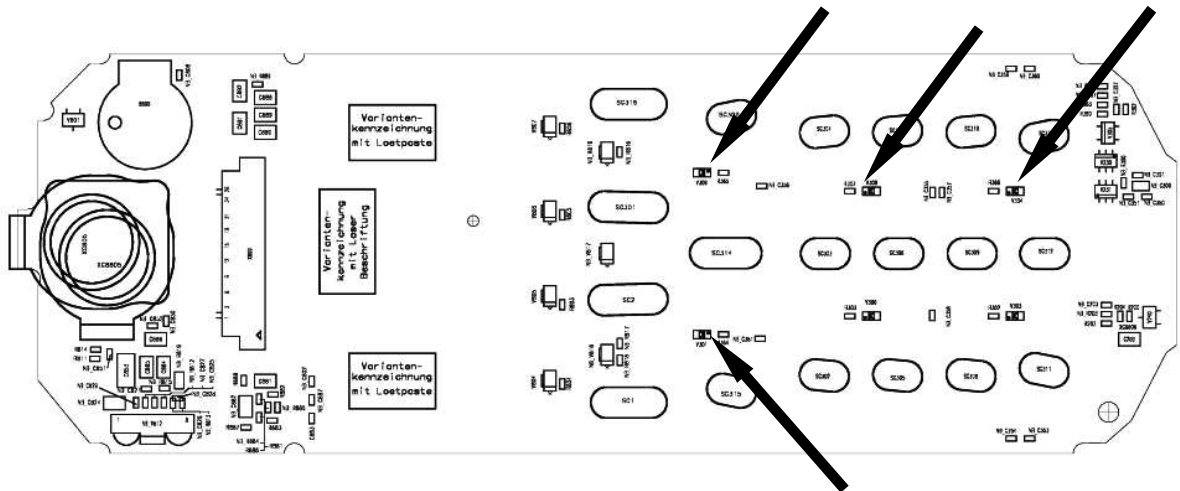
Figure 2: X35 keyboard LED placement and polarity (top view)
