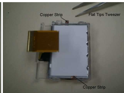
PHOTO 2.18 Disassembly Display Module – STEP 1
