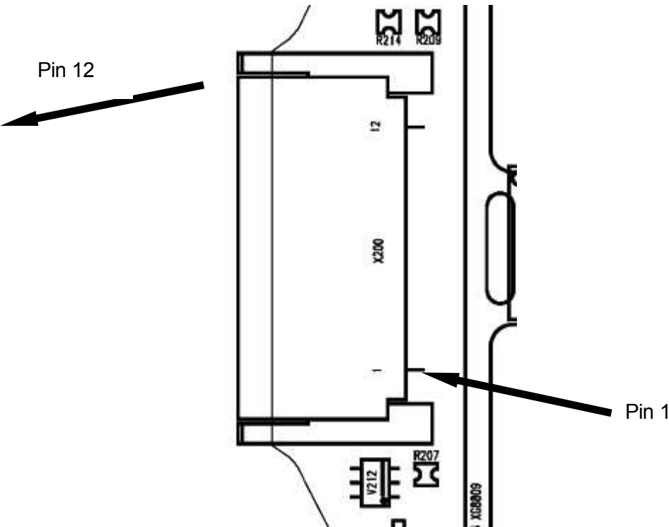
Figure 2: X35 Bottom Connector Placement (Top View)
