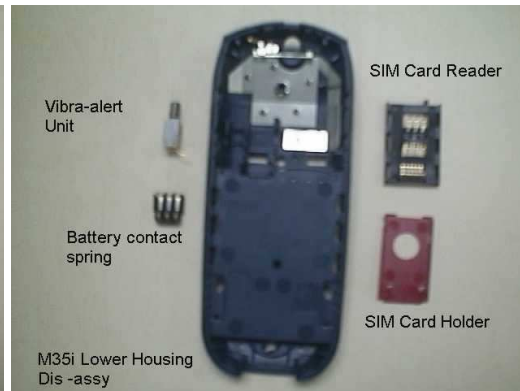
PHOTO 2.13 Disassembly Lower Housing – STEP 2
