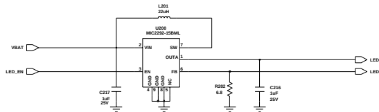
LCD BACKLIGHT
